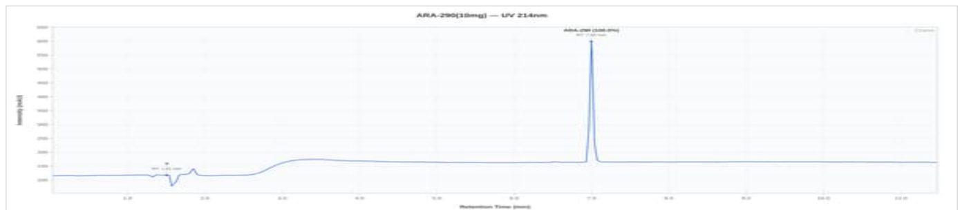
Ara-290 10mg - 2107: UV Chromatogram
