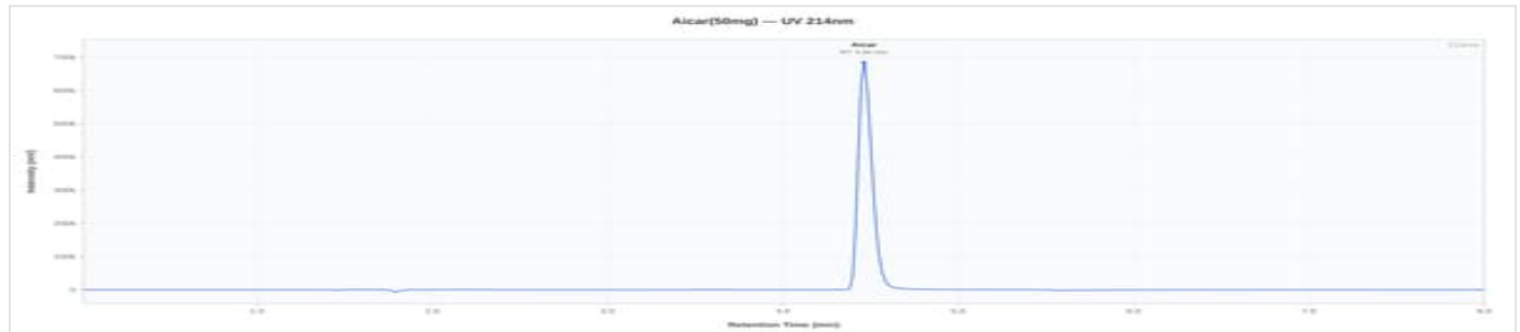
AICAR 50mg - 2107: UV Chromatogram
